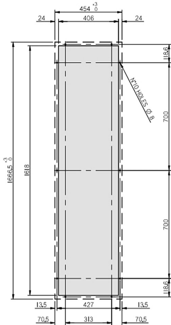
MONTAGGIO A INCASSO / SEMINCASSO FLUSH / SEMI-FLUSH MOUNTING
